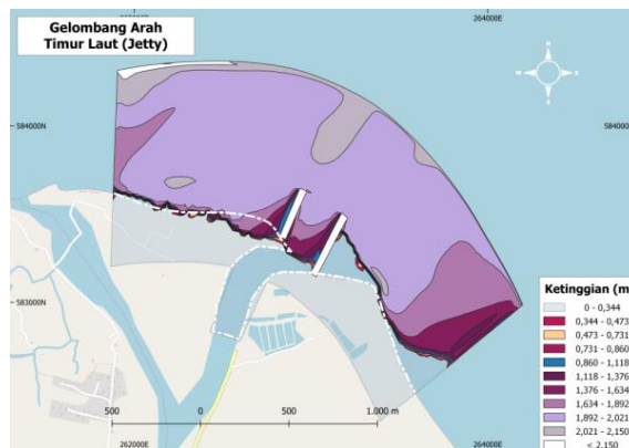
Figure 8. Wave Modeling of North East Wind Direction
