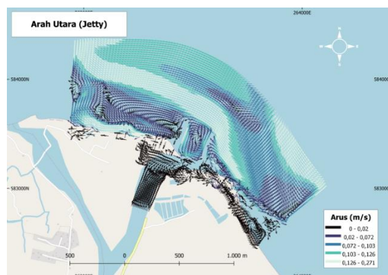
Figure 6. Current Pattern of North Wind Direction
