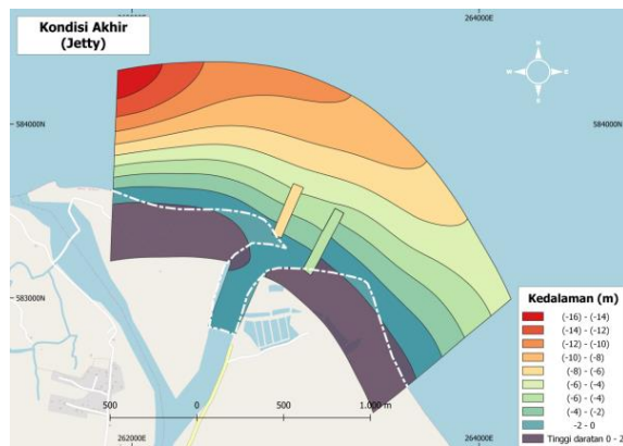
Figure 10. Beach Morphology Conditions with Modeling
