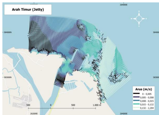
Figure 3. Current Pattern of East Wind Direction
