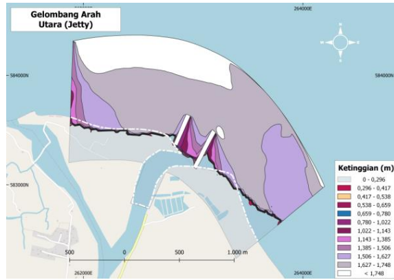
Figure 9. Wave Modeling of North East Wind Direction
