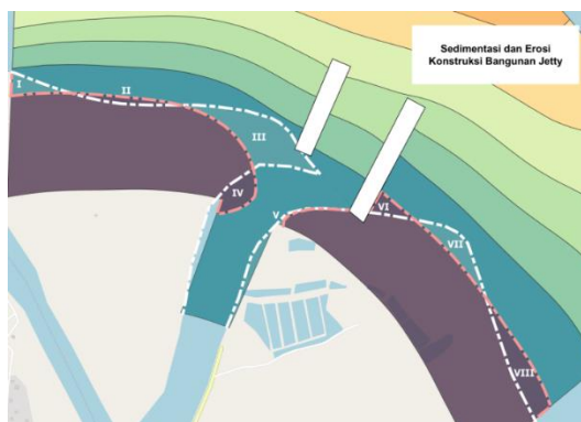
Figure 11. Erosion and Sedimentation Areas
