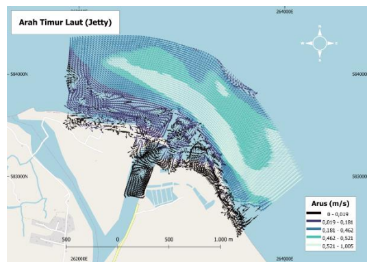
Figure 5. Current Pattern of North East Wind Direction
