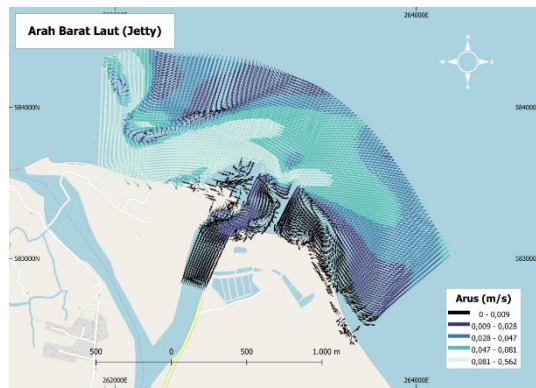
Figure 4. Current Pattern of North West Wind Direction
